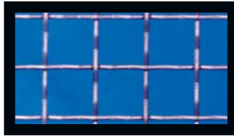
1-5/8" center-to-center square 8 gauge (1-1/2" square opening)
